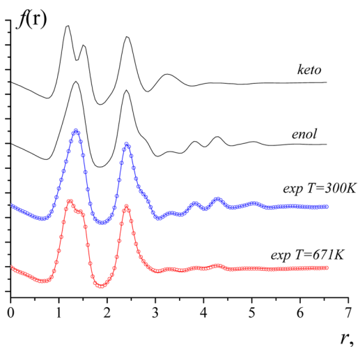
Figure 2. Experimental (dots) and calculated radial distribution functions for two experimental series at two temperatures and the theoretical curves for two tautomeric forms.
